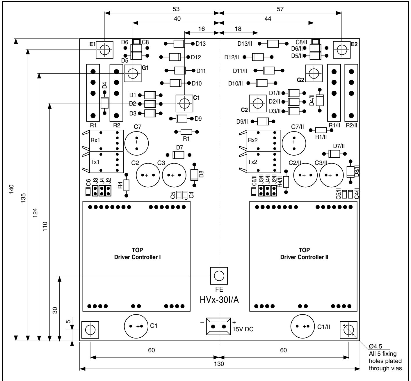
Fig. 2 Outline details
